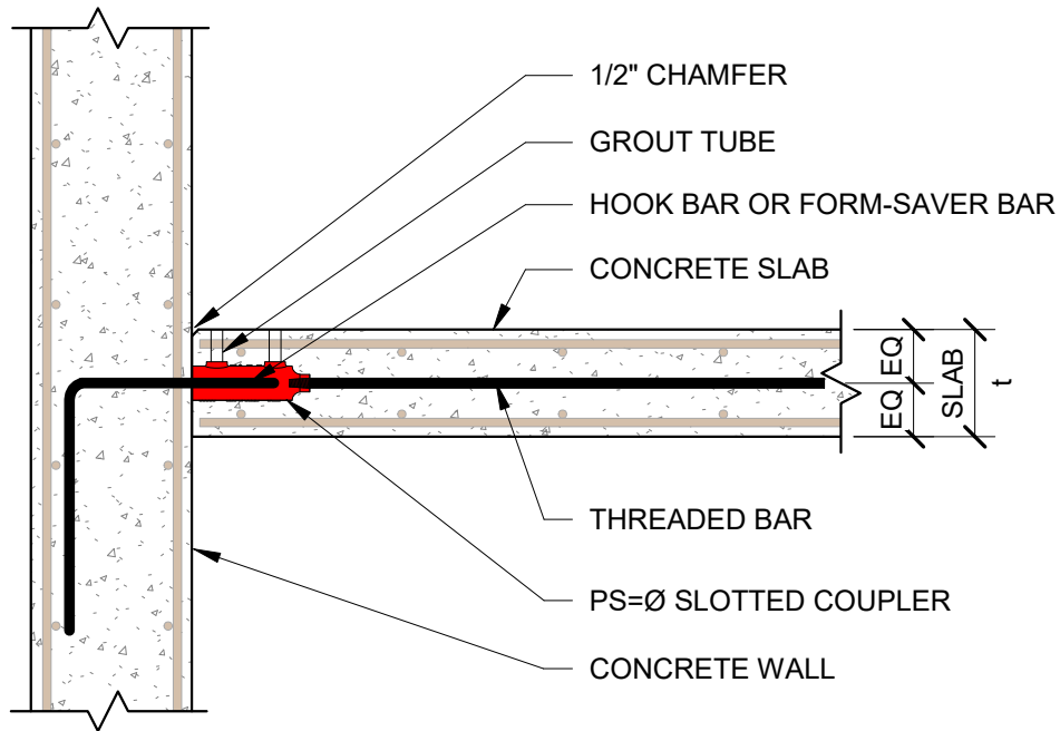
1 SLAB RELIEF JOINT @ WALL 3/4" = 1'-0"
