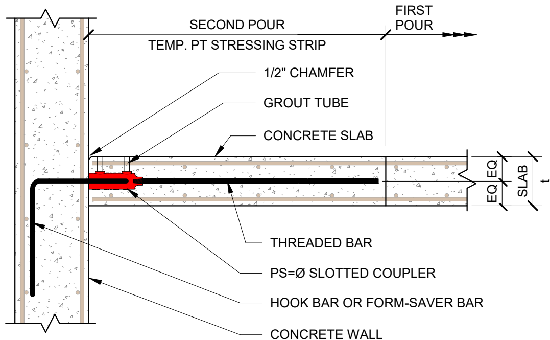
2 SLAB RELIEF JOINT @ WALL w/TEMP. PT STRESSING STRIP 3/4" = 1'-0"
